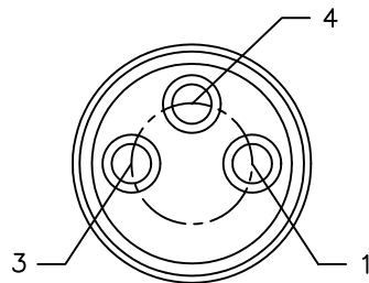
MATING FACE – SOCKET INSERT (PIN INSERT POSITIONS OPPOSITE)
