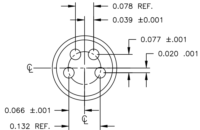
WIRING VIEW
