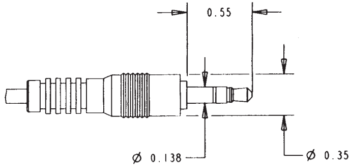
END CODE: 35 3.5 mm STRAIGHT PLUG
