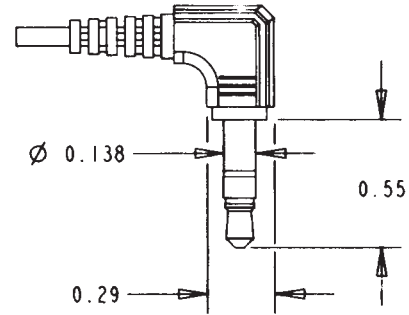
END CODE: 36 3.5 mm RIGHT-ANGLE PLUG
