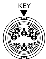
WIRING END W6880-8PG-P-5XX
