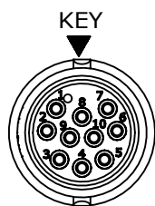
SHOWN ASSEMBLED KIT ASSY: W6880-10PG-P-5XX SHOWN
