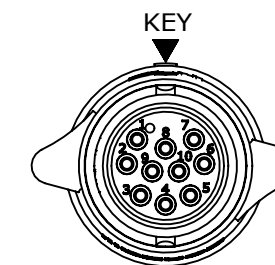
WIRING END ASSY: W6880-10PG-P-5XX SHOWN WITHOUT HARDWARE
