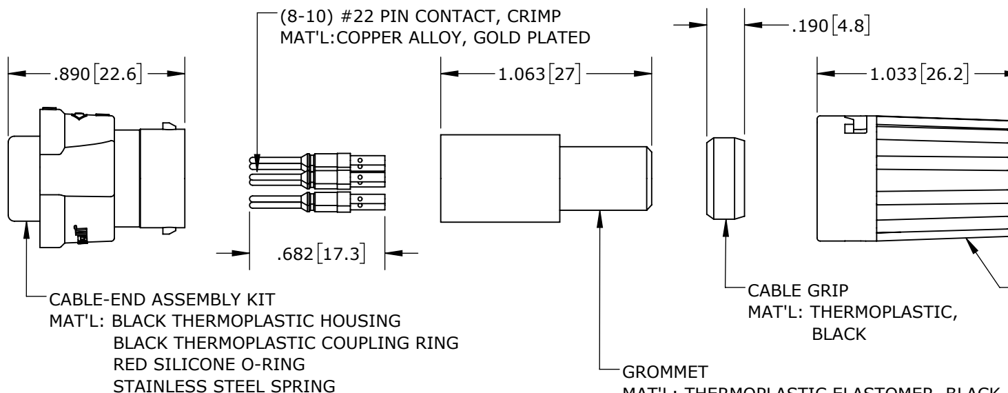
BACKSHELL MAT'L: THERMOPLASTIC, BLACK
