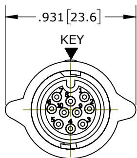
MATING FACE ASSY: W6880-10PG-P-5XX SHOWN
