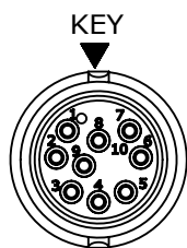
WIRING END W6880-9PG-P-5XX
