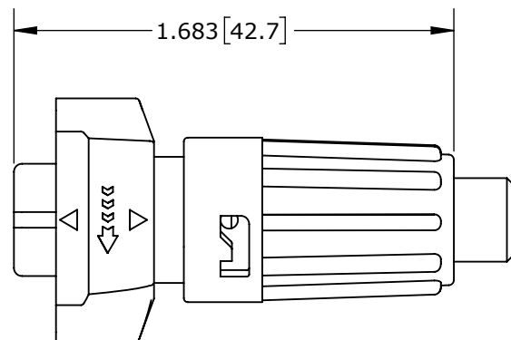
SHOWN ASSEMBLED KIT ASSY: W6380-2PG-P-5XX SHOWN
