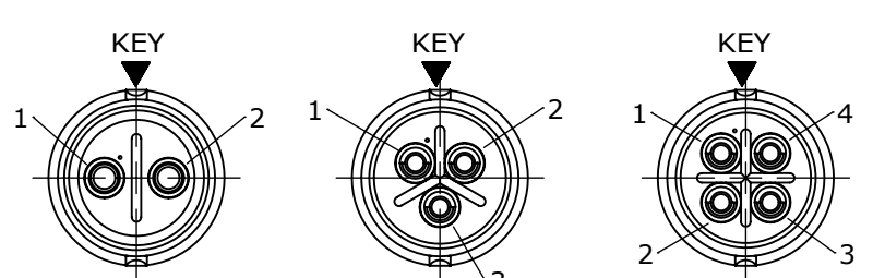
WIRING END W6380-2PG-P-5XX WIRING END W6380-3PG-P-5XX WIRING END W6380-4PG-P-5XX
