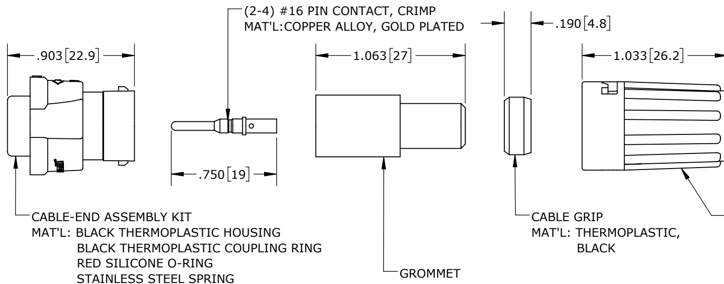
SHOWN ASSEMBLED KIT ASSY: W6380-2PG-P-5XX SHOWN
