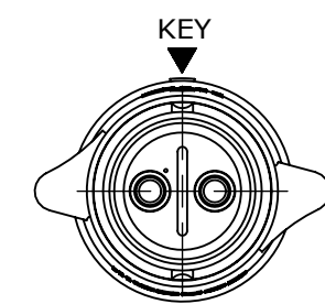
WIRING END ASSY: W6380-2PG-P-5XX SHOWN WITHOUT HARDWARE
