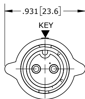
MATING FACE ASSY: W6380-2PG-P-5XX SHOWN
