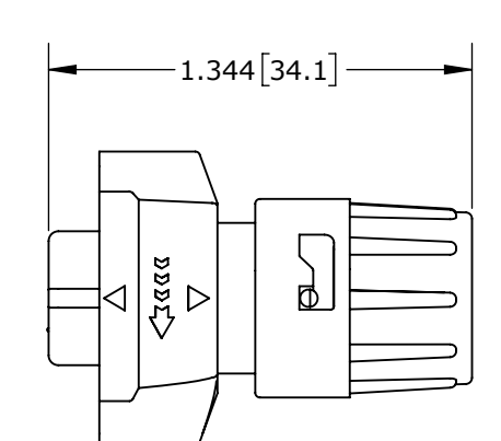
SHOWN ASSEMBLED KIT ASSY: W6282-2SG-P-3XX SHOWN
