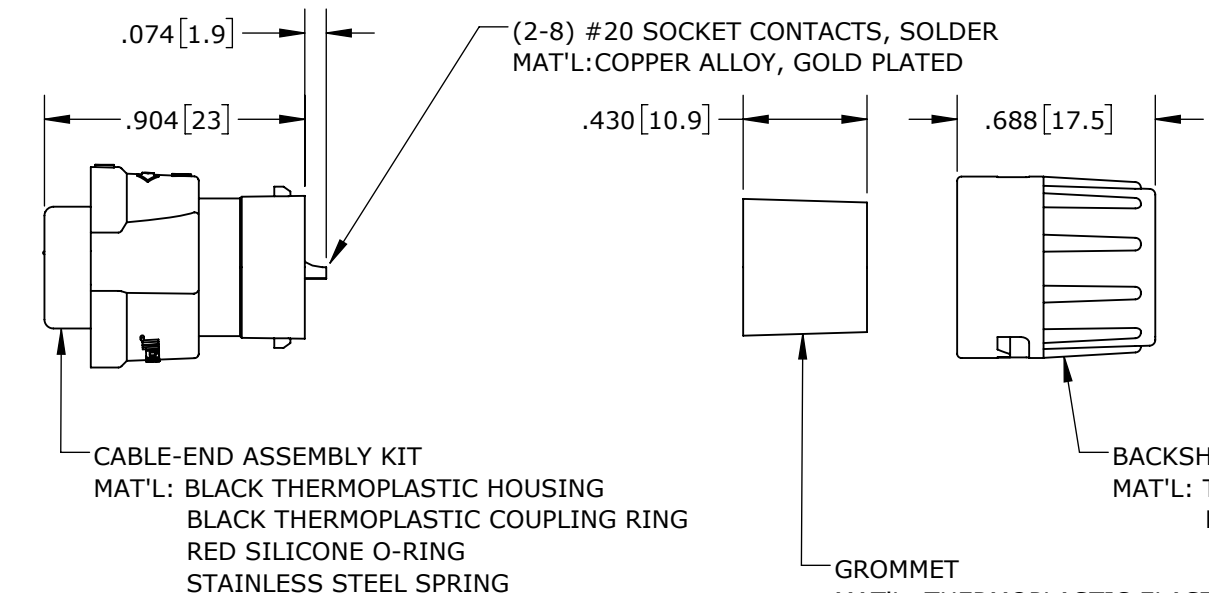
SHOWN ASSEMBLED KIT ASSY: W6282-2SG-P-3XX SHOWN
