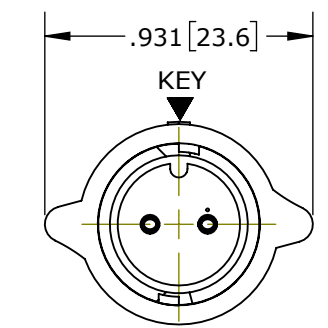
MATING FACE ASSY: W6282-2SG-P-3XX SHOWN
