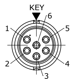
WIRING END W6282-6PG-P-3XX
