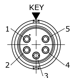
WIRING END W6282-5PG-P-3XX
