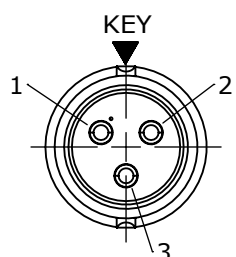
WIRING END W6282-3PG-P-3XX
