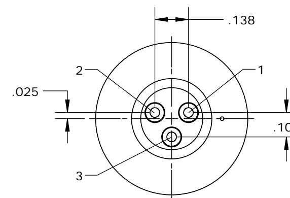
WIRE VIEW 17292-3PG-300
