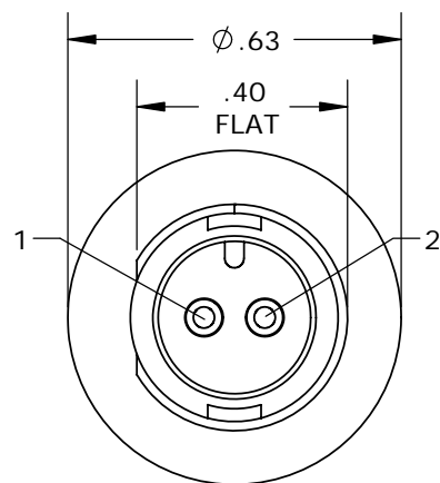
FACE VIEW 17292-2PG-300
