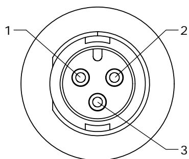
FACE VIEW 17292-3PG-300
