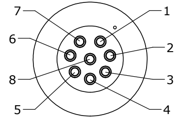
WIRING END ASSY: W7280-8PG-300
