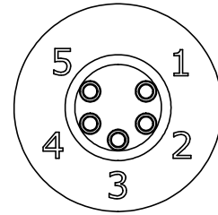
WIRING END ASSY: W7280-5PG-300
