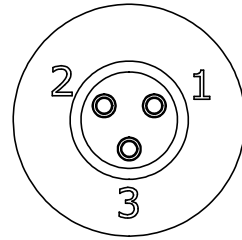
WIRING END ASSY: W7280-3PG-300
