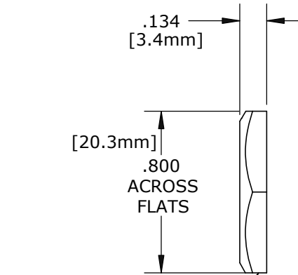
HEX NUT MAT'L: UV PBT, BLACK
