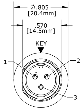
MATING FACE ASSY: W7280-3PG-300 SHOWN
