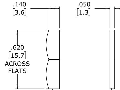
HEX NUT MAT'L: NEOPRENE, BLACK GASKET
