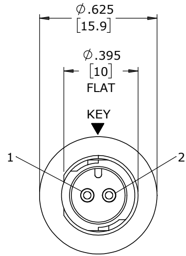
FACE VIEW W17292-2PG-P-3ES MAT'L: UV PBT, BLACK
