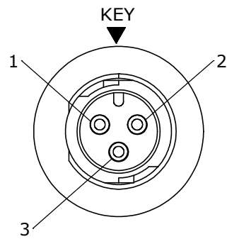
FACE VIEW W17292-3PG-P-3ES
