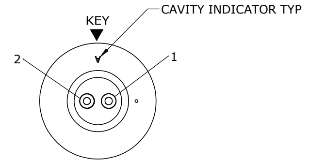
WIRE VIEW W17292-2PG-P-3ES
