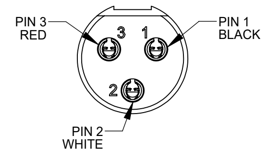
ST-603 FRONT MATING VIEW
