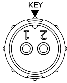
FACE VIEW ASSY: 5180-2PG-3XX
