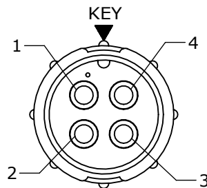
FACE VIEW ASSY: 5180-4PG-3XX
