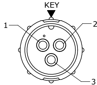
FACE VIEW ASSY: 5180-3PG-3XX
