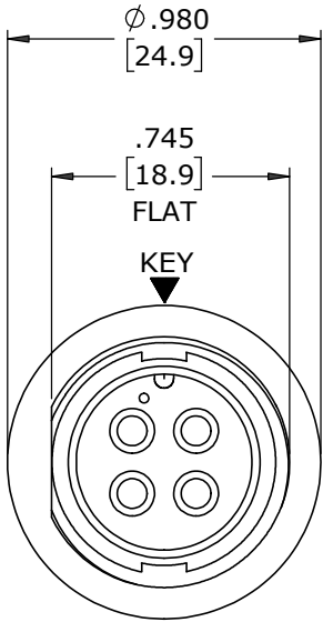
FACE VIEW 4181-4PG-3ES SHOWN
