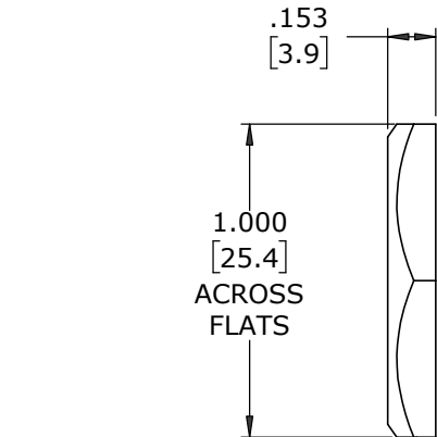
HEX NUT MAT'L: NYLON, BLACK
