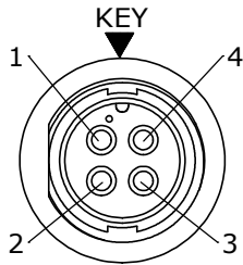
FACE VIEW 4181-4PG-3ES
