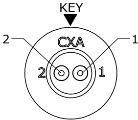
WIRE VIEW 4181-2PG-3ES
