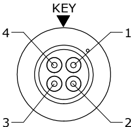
WIRE VIEW 4181-4PG-3ES
