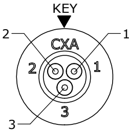
WIRE VIEW 4181-3PG-3ES
