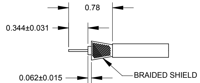
RECOMMENDED CABLE STRIPPING DETAIL
