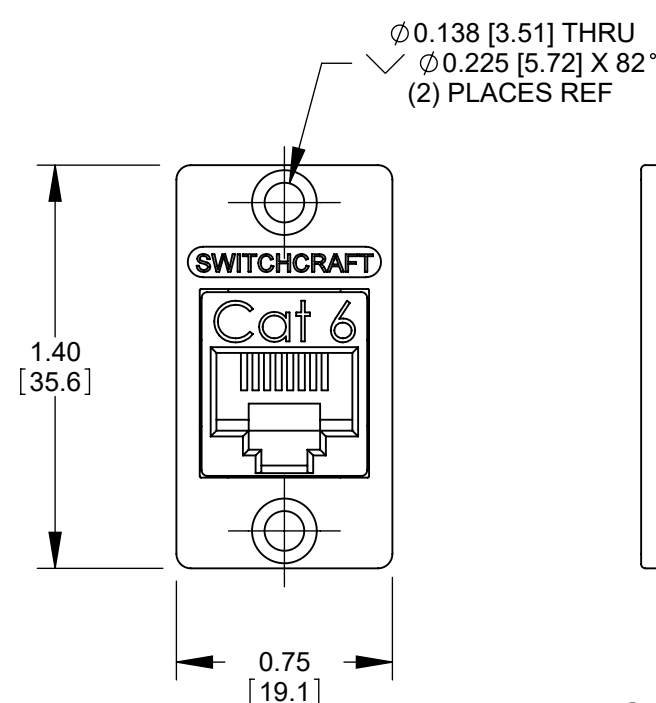
NHRJ45D6B - UNSHIELDED (SHOWN) NHRJ45D6S - SHIELDED
