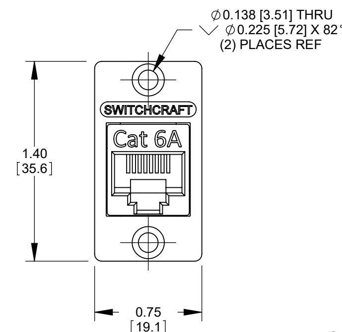
NHRJ45D6AB - UNSHIELDED (SHOWN) NHRJ45D6AS - SHIELDED
